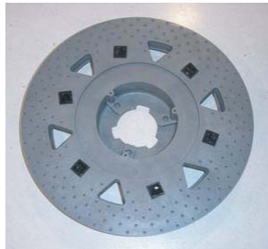
17" Pad Driver 17" round spike plate that accommodates fiber pads for polishing and scrubbing.
